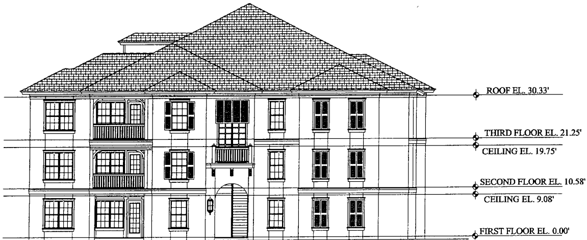
② BUILDING TYPE TWO - RIGHT ELEVATION
