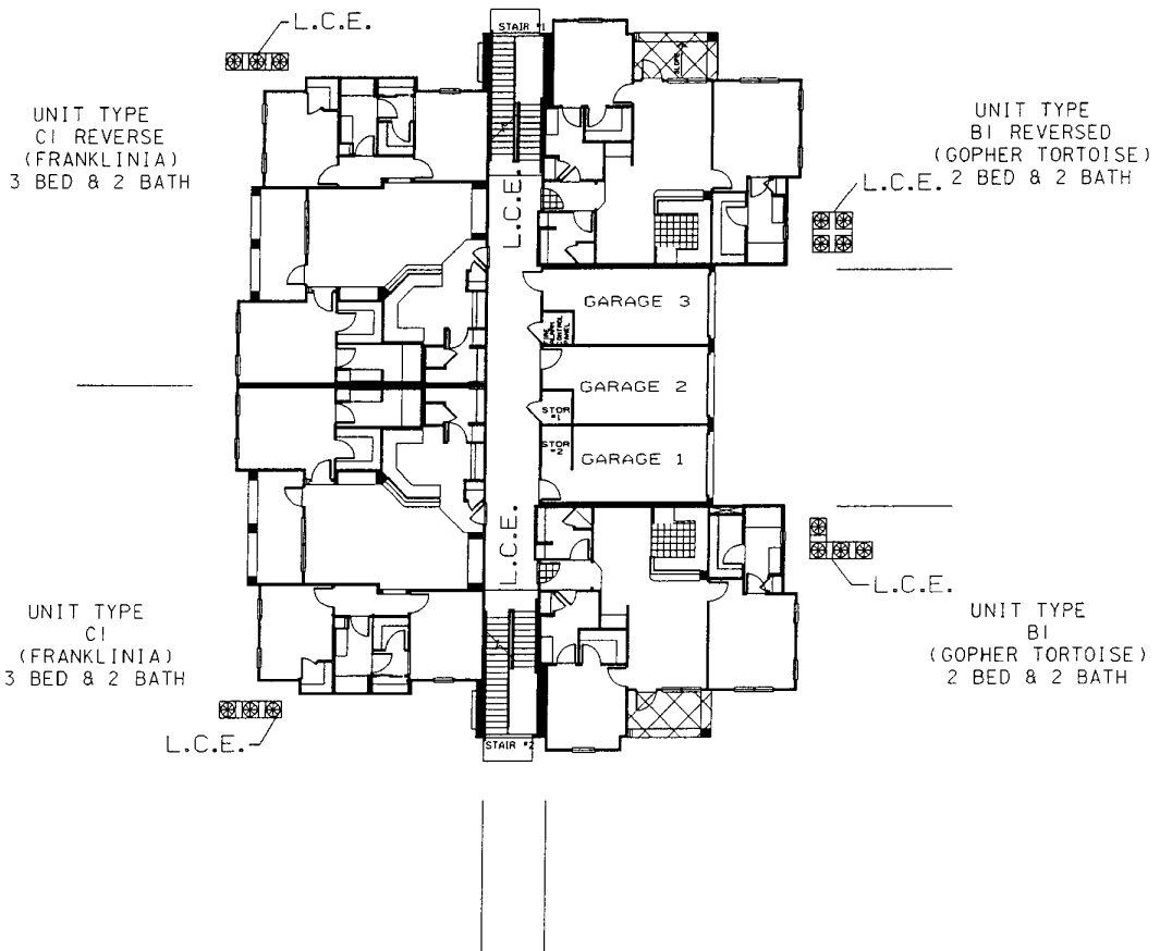
BUILDING #2 - FIRST FLOOR PLAN
