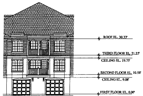
① BUILDING TYPE ONE - PARTIAL SIDE ELEVATION
