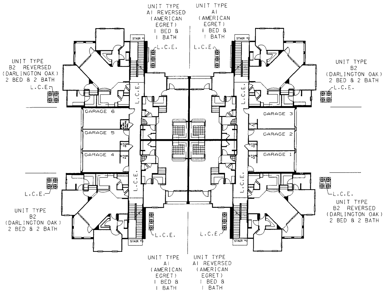
BUILDING #1 - FIRST FLOOR PLAN
