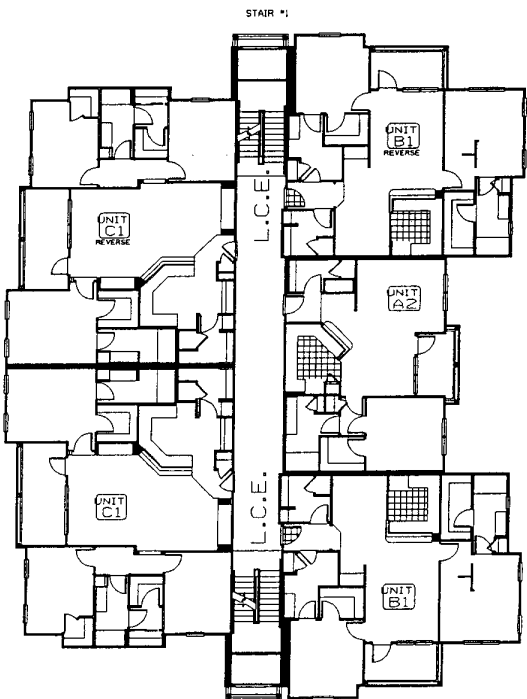
BUILDING #2 - THIRD FLOOR PLAN
