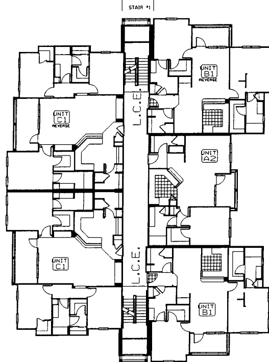
BUILDING #2 - SECOND FLOOR PLAN
