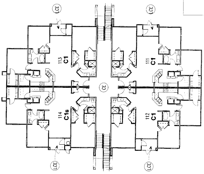
FIRST FLOOR BUILDING TYPE V
