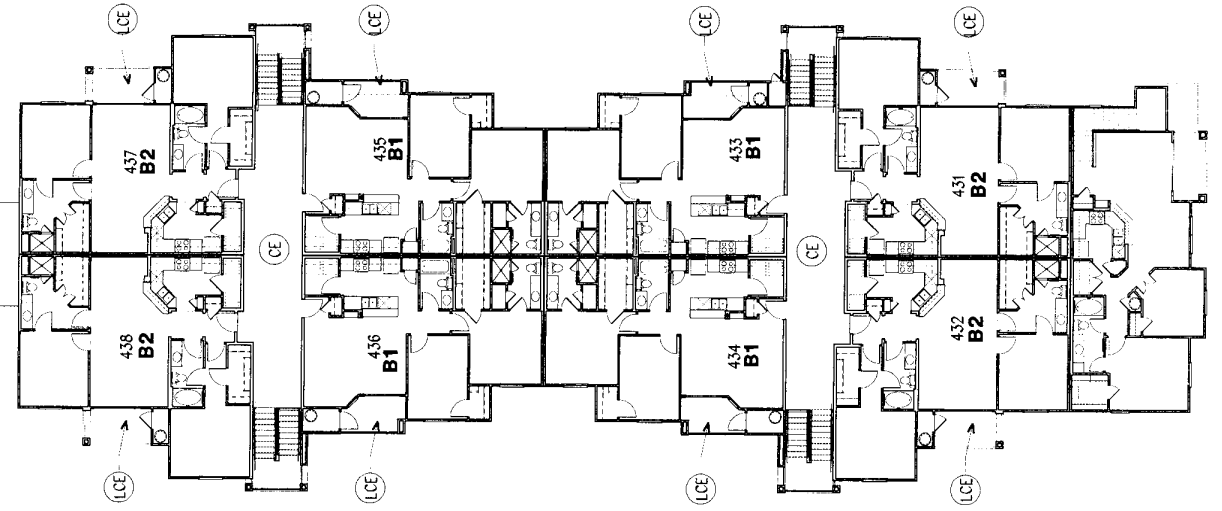
THIRD FLOOR BUILDING TYPE III
