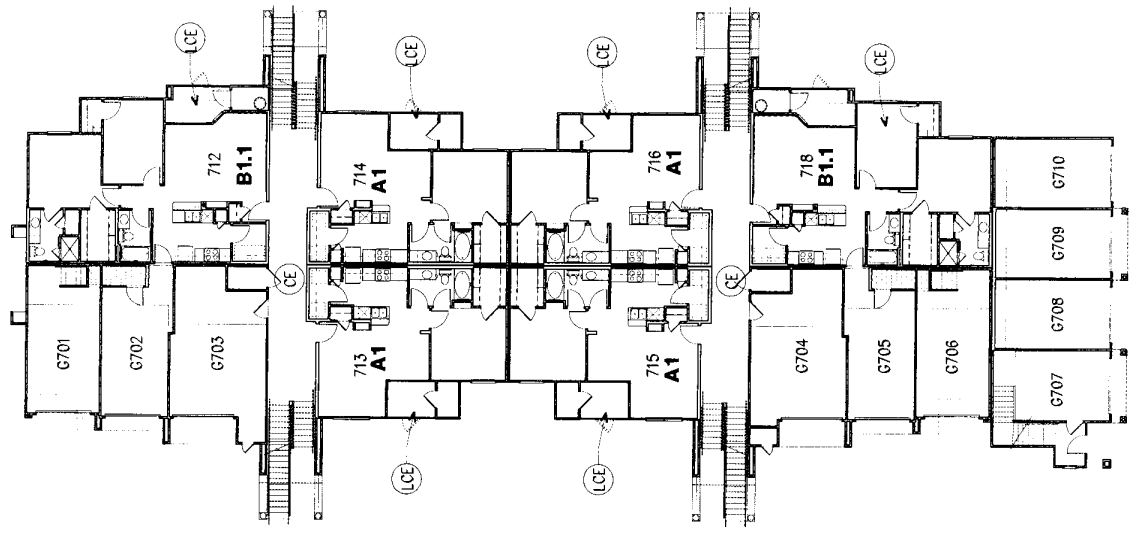
FIRST FLOOR BUILDING TYPE 1A
