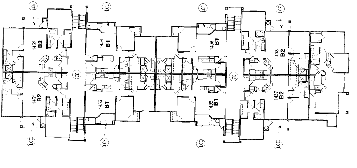
THIRD FLOOR BUILDING TYPE III
