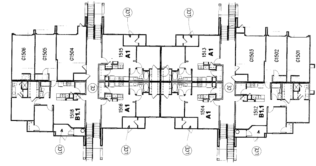
FIRST FLOOR BUILDING TYPE 1
