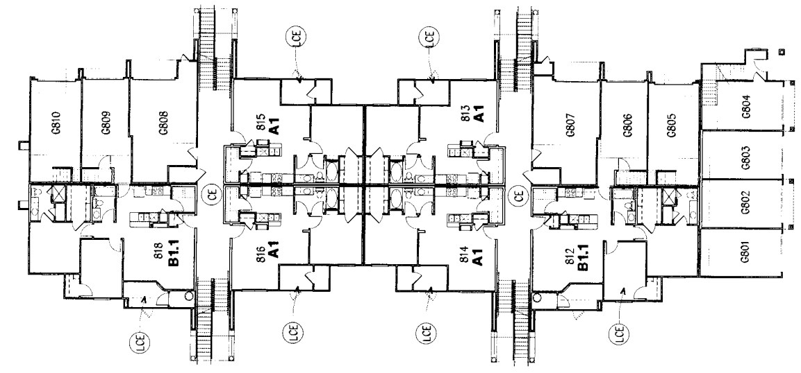
FIRST FLOOR BUILDING TYPE IA
