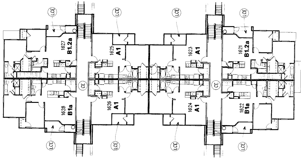
SECOND FLOOR BUILDING TYPE I
