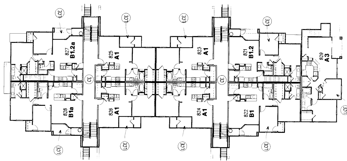
SECOND FLOOR BUILDING TYPE IA
