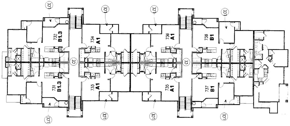
THIRD FLOOR BUILDING TYPE 1A
