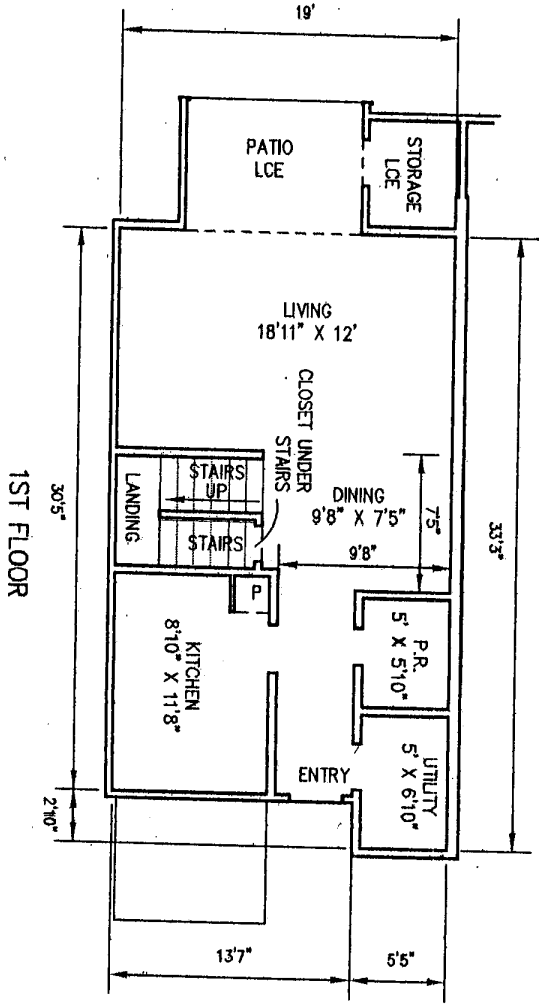
2 BEDROOM/2-1/2 BATH TOWNHOUSE
