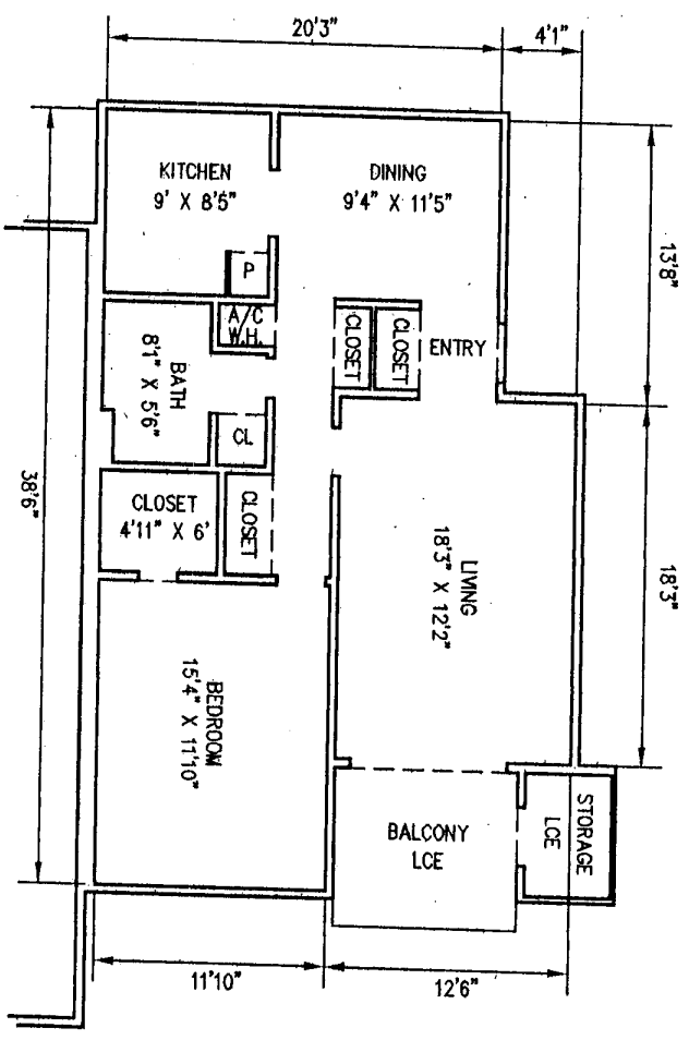
1 BEDROOM/1 BATH FLOOR PLAN (LARGE) 2ND FLOOR UNITS
