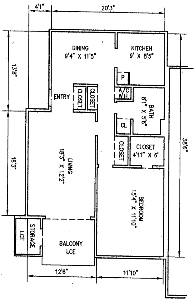
1 BEDROOM/1 BATH FLOOR PLAN (LARGE) (REVERSE) 2ND FLOOR UNITS
