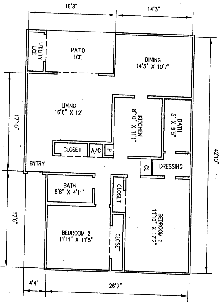
2 BEDROOM/2 BATH FLOOR PLAN (REVERSE) 1ST FLOOR UNITS
