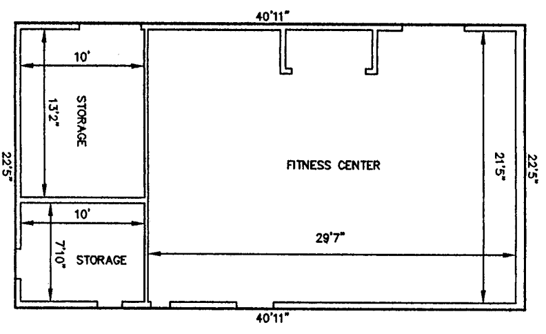
FITNESS CENTER AND STORAGE BUILDING
