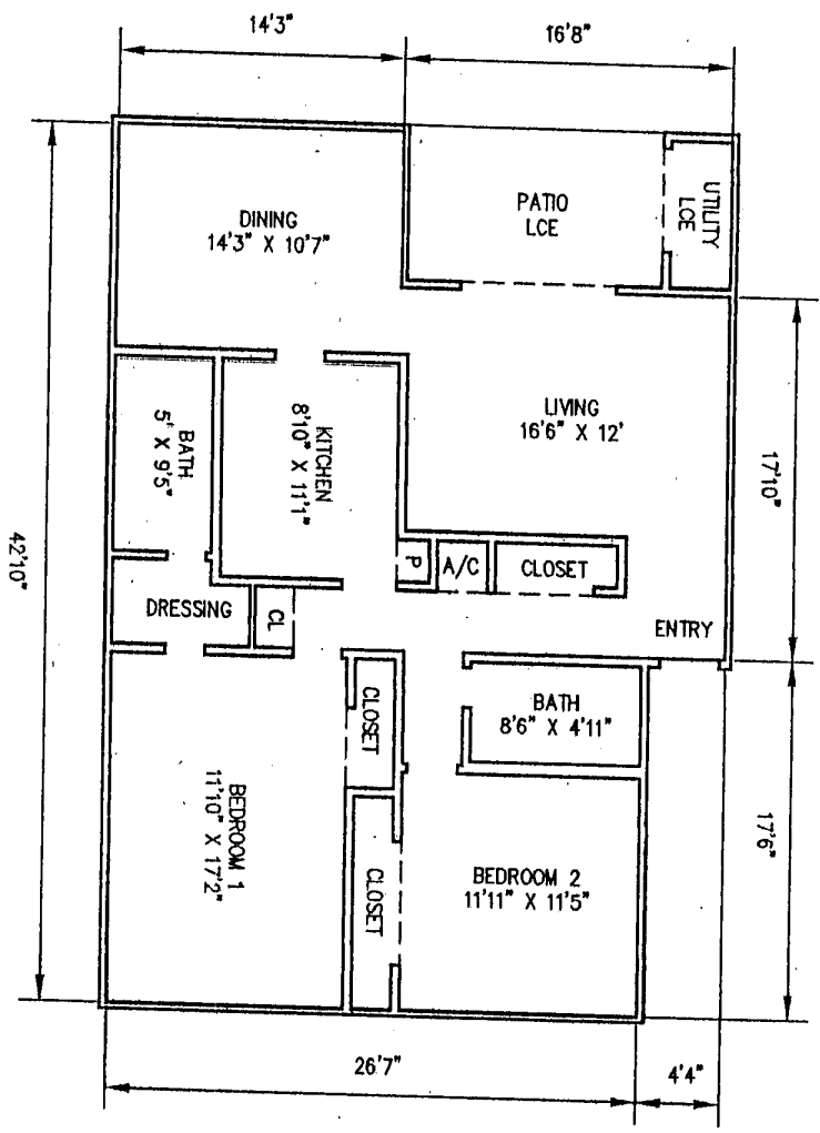
2 BEDROOM/2 BATH FLOOR PLAN 1ST FLOOR UNITS
