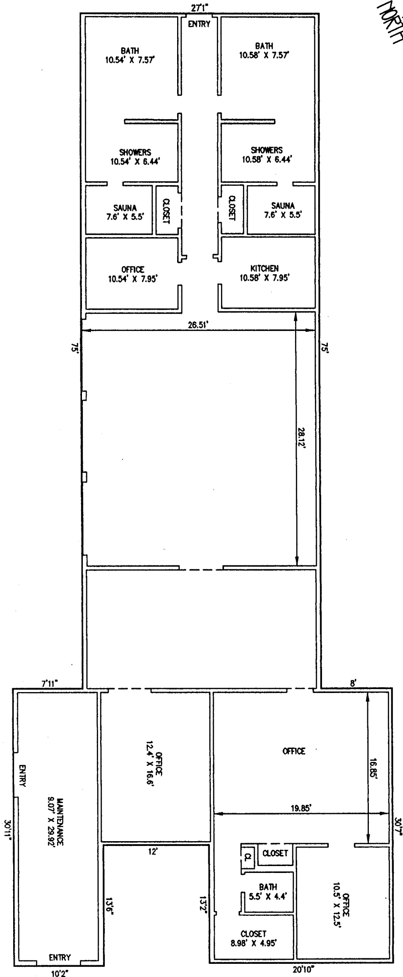
CLUBHOUSE AND MAINTENANCE BUILDING
