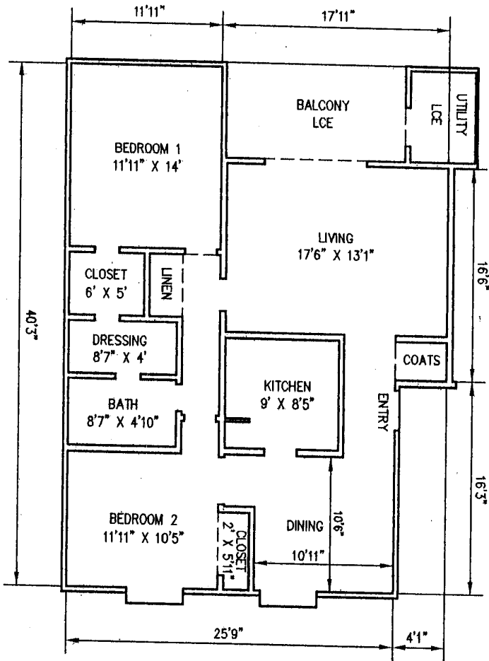
2 BEDROOM/1 BATH FLOOR PLAN 2ND FLOOR UNITS
