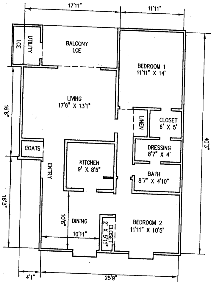
2 BEDROOM/1 BATH FLOOR PLAN (REVERSE) 2ND FLOOR UNITS
