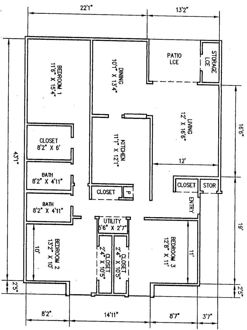
3 BEDROOM/2 BATH FLOOR PLAN 1ST FLOOR UNITS
