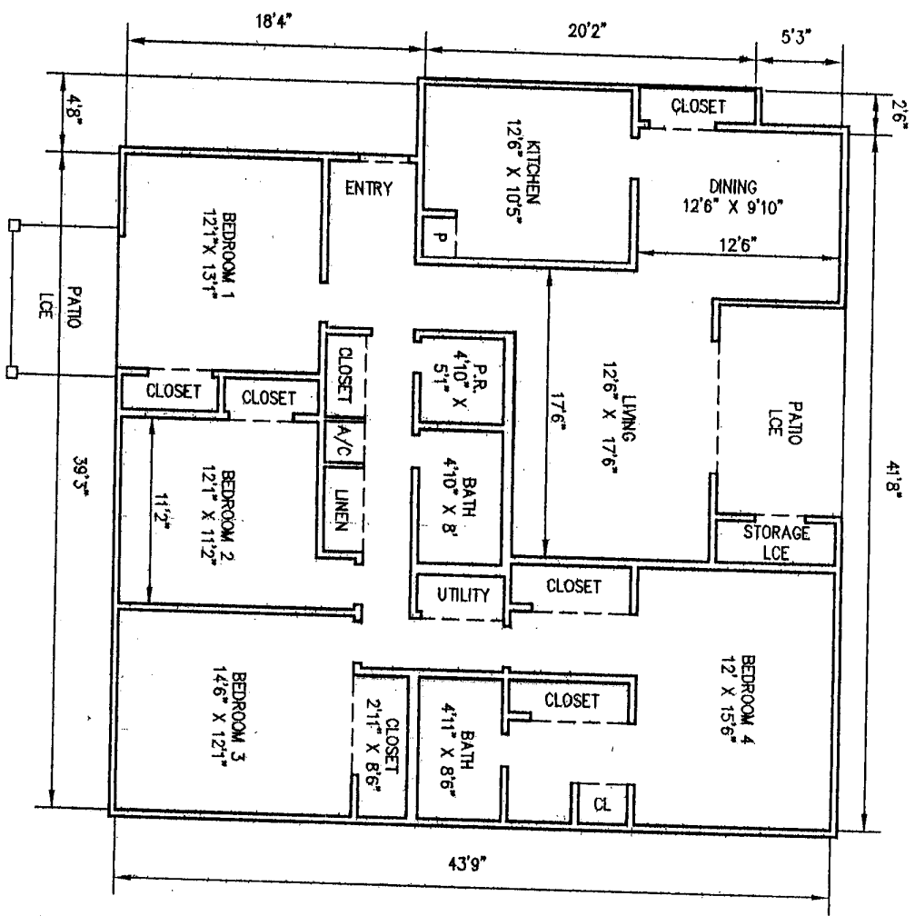
4 BEDROOM/2-1/2 BATH FLOOR PLAN 1ST FLOOR UNITS
