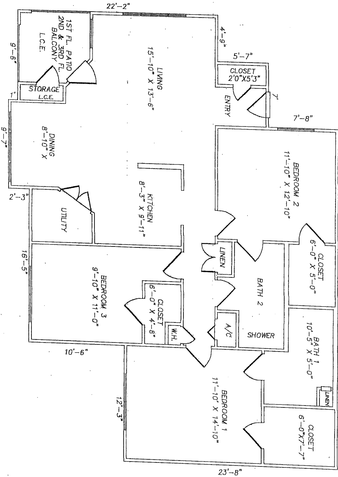
UNIT F--REVERSE FLOOR PLAN
