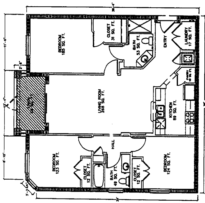
FLOOR PLAN UNIT "B-1"
