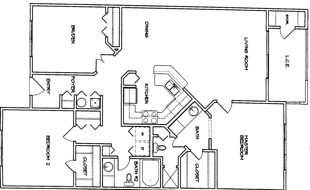
3 THREE BEDROOM UNIT (CE) FLOOR PLAN 1/8" = 1'-0"
