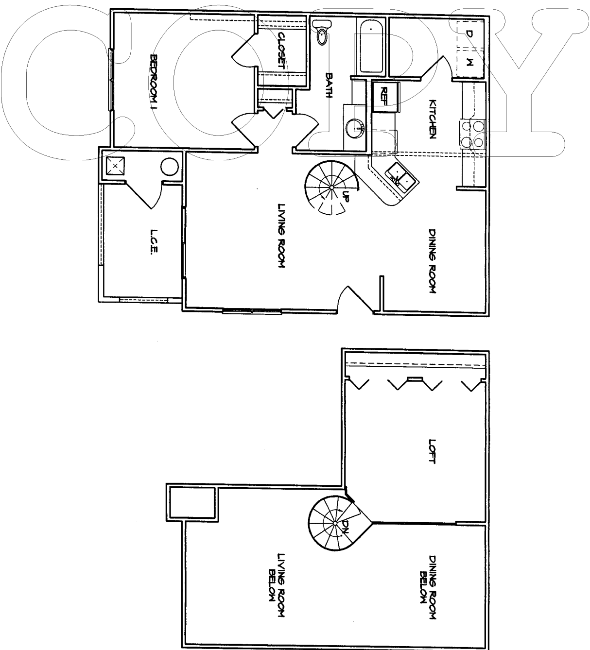
2 ONE BEDROOM UNIT (A1) FLOOR PLAN WITH LOFT A-4 1/8" = 1'-0"
