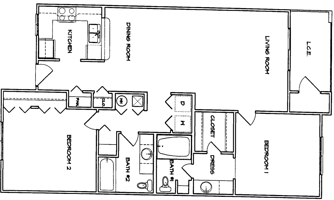
6 TWO BEDROOM UNIT (BE) FLOOR PLAN A-4 1/8" = 1'-0"
