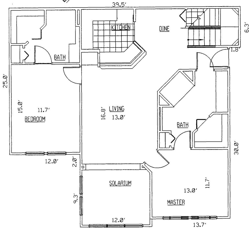
② UNIT TYPE S2L 2 BEDROOM FLOOR PLAN, LOFT W/ SOLARIUM UNIT NUMBERS 1533, 1633.
