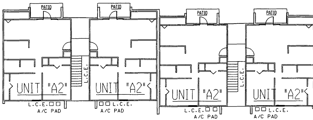
VII BUILDING TYPE VII - FIRST FLOOR PLAN
