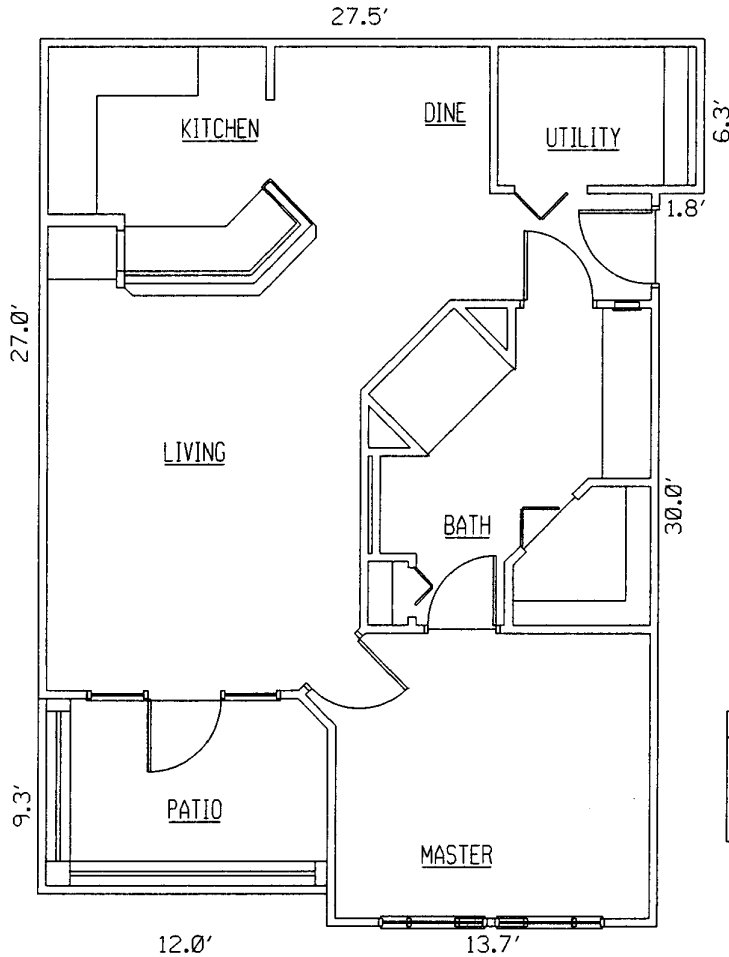
1 UNIT TYPE P1 1 BEDROOM FLOOR PLAN W/ PATIO
