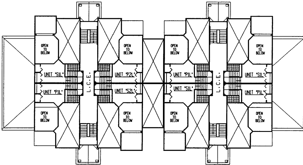
1 BUILDING TYPE I FOURTH FLOOR PLAN
