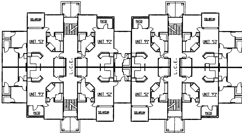
① BUILDING TYPE I SECOND FLOOR PLAN
