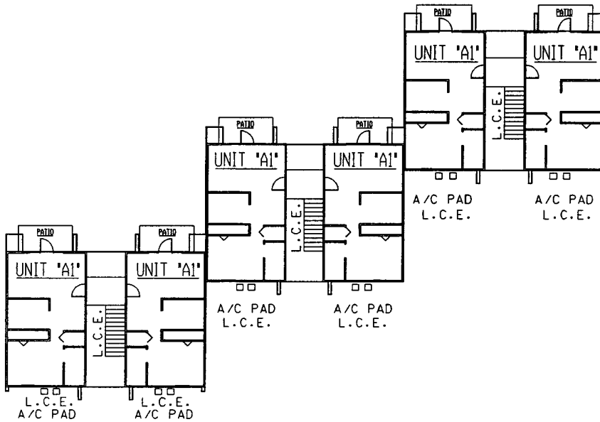
VI BUILDING TYPE VI - FIRST FLOOR PLAN BUILDING TYPE VI BUILDING 5
