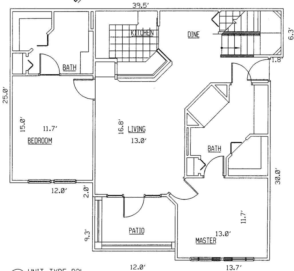
2 UNIT TYPE P2L 2 BEDROOM FLOOR PLAN, LOFT W/ PATIO
