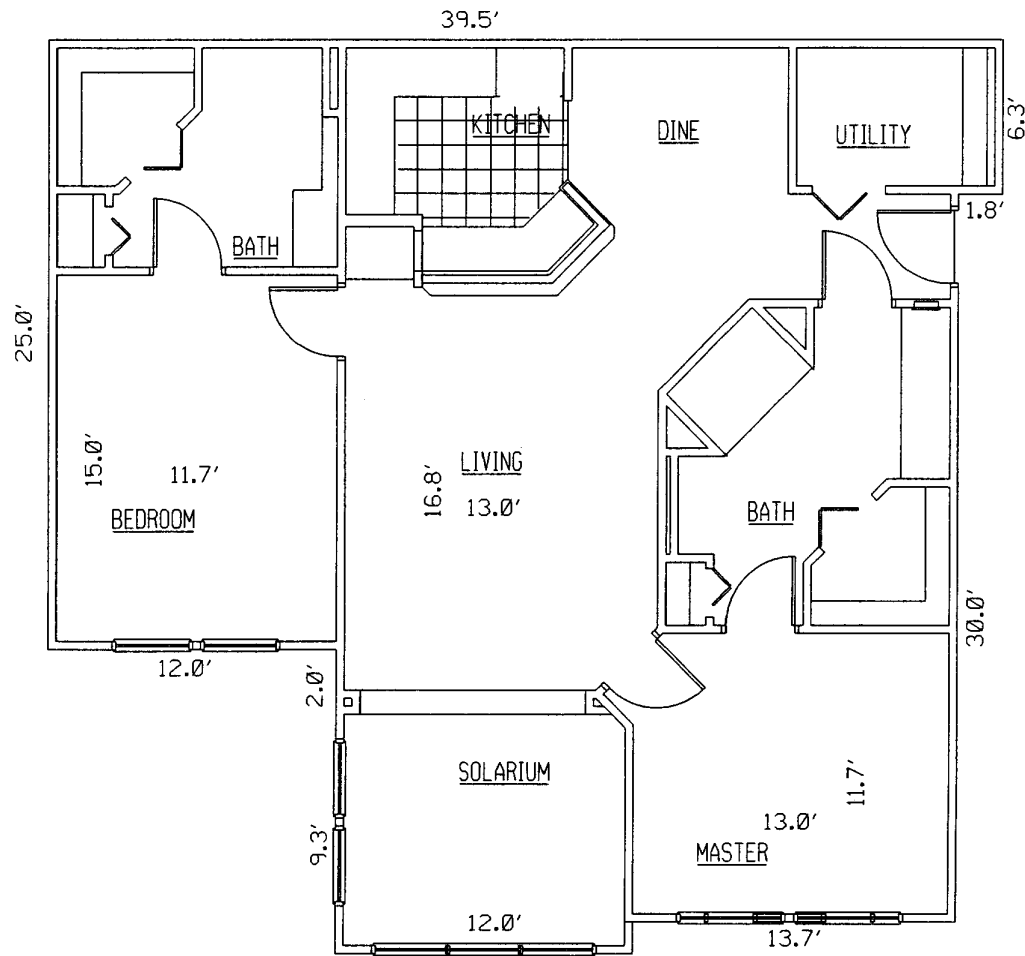
② UNIT TYPE S2 2 BEDROOM 2 BATH FLOOR PLAN W/ SOLARIUM
