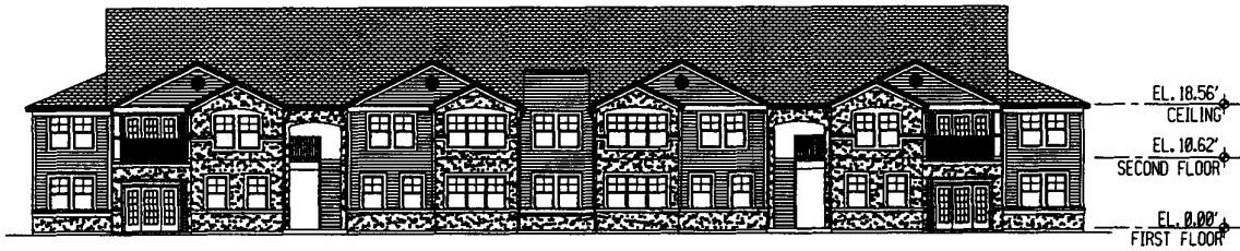
① BUILDING TYPE II - FRONT ELEVATION
