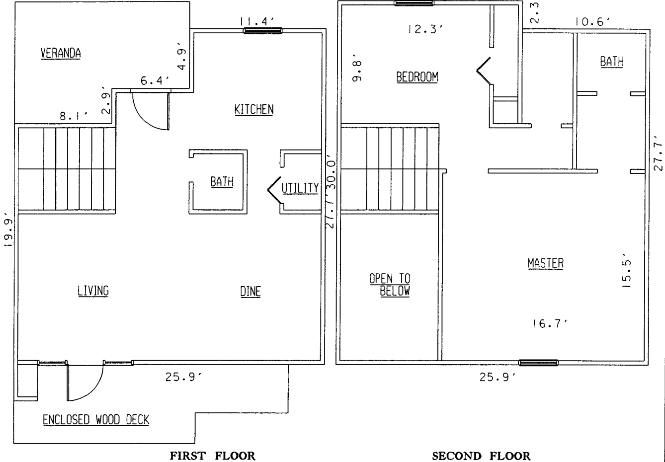
② UNIT TYPE D2 TOWNHOME 2 BEDROOM FLOOR PLAN W/ DECK
