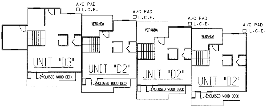
III BUILDING TYPE III - FIRST FLOOR PLAN
