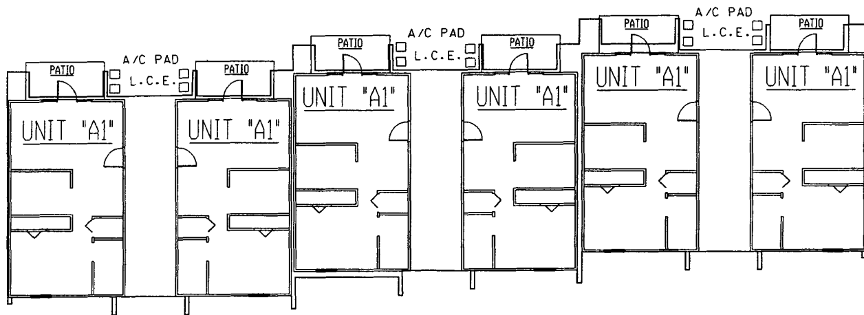
VIII BUILDING TYPE VIII - FIRST FLOOR PLAN
