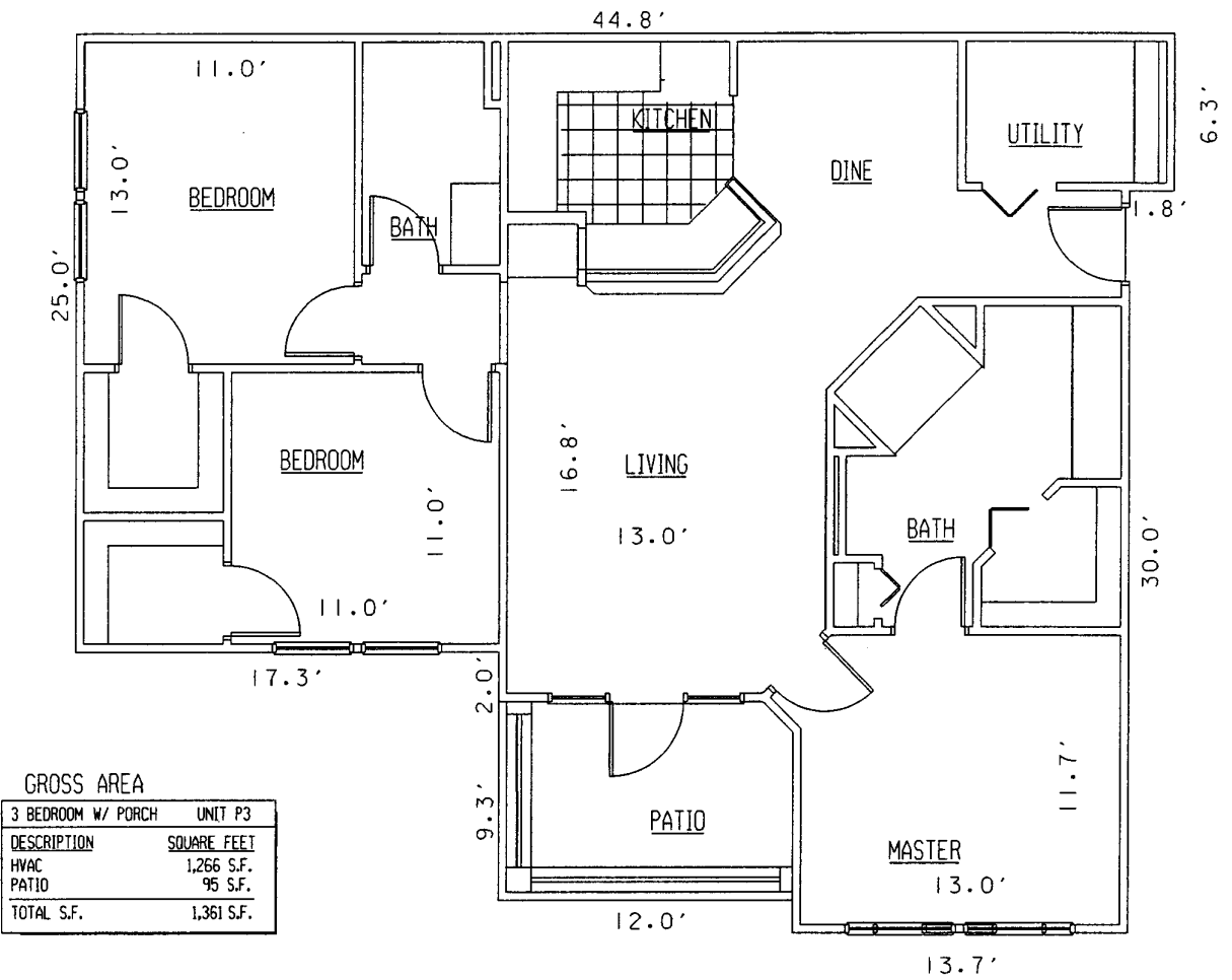
3 UNIT TYPE P3 3 BEDROOM FLOOR PLAN W/ PORCH
