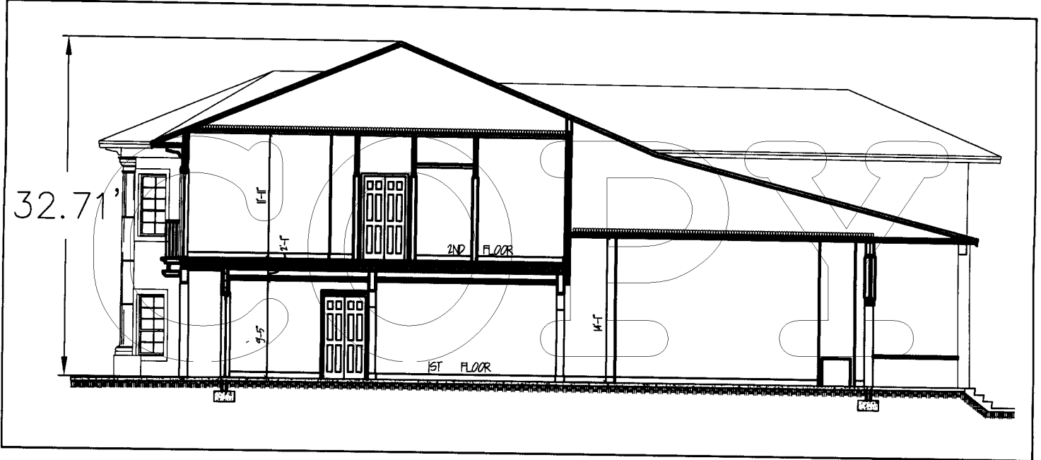
BUILDING SECTION
