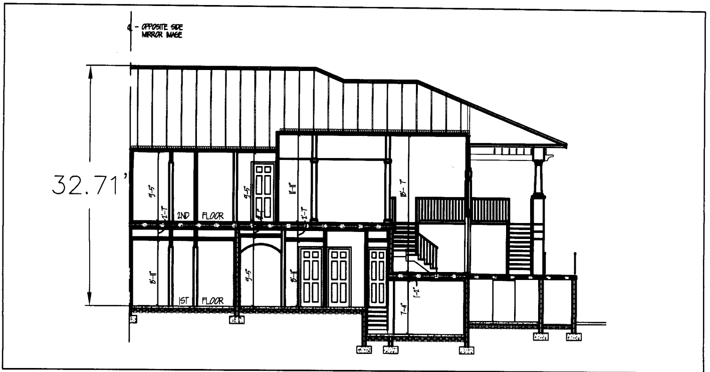
BUILDING SECTION
