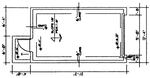
FOUNDATION PLAN
