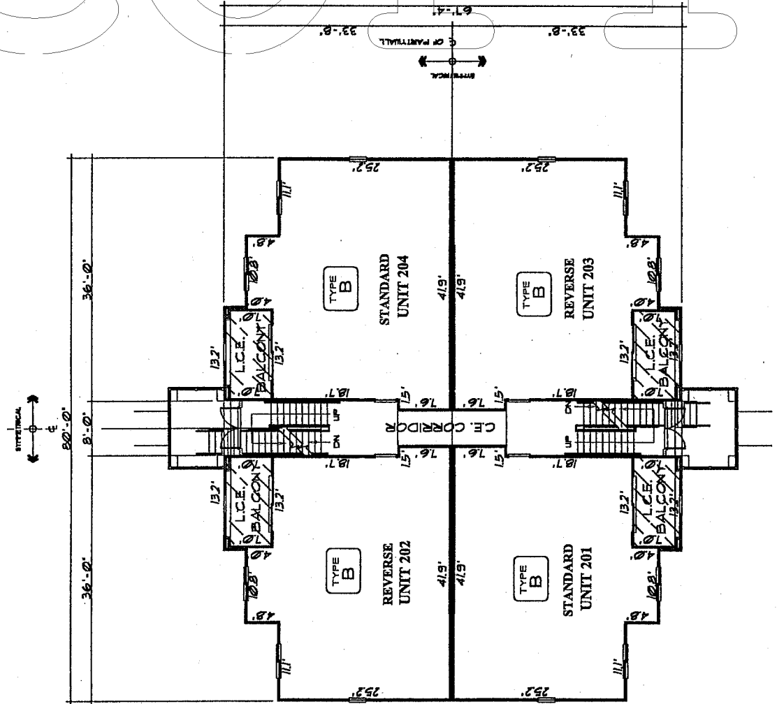
BUILDING 625 (TYPICAL FLOOR PLAN) BUILDING TYPE #2 - SECOND FLOOR - FLOOR PLAN
