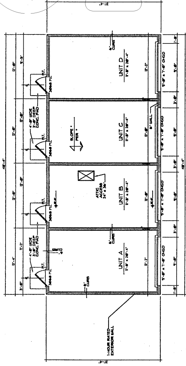
BUILDINGS GARAGE No. 2, 3 AND 5 THROUGH 14 GARAGE TYPE #4 - FLOOR PLAN (SEE SITE PLAN FOR STRUCTURES LOCATION)
