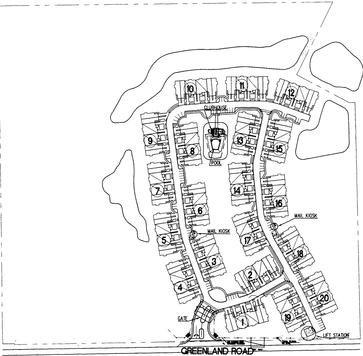
1"=200'-0" ① SITE PLAN
