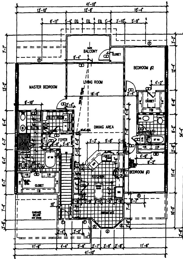
3/32" = 1'-0" 1 SECOND FLOOR PLAN UNIT D - DARLINGTON - 3BR FLAT RIGHT UNIT 05
