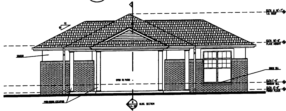
3/32" = 1'-0" 2 SOUTH ELEVATION
