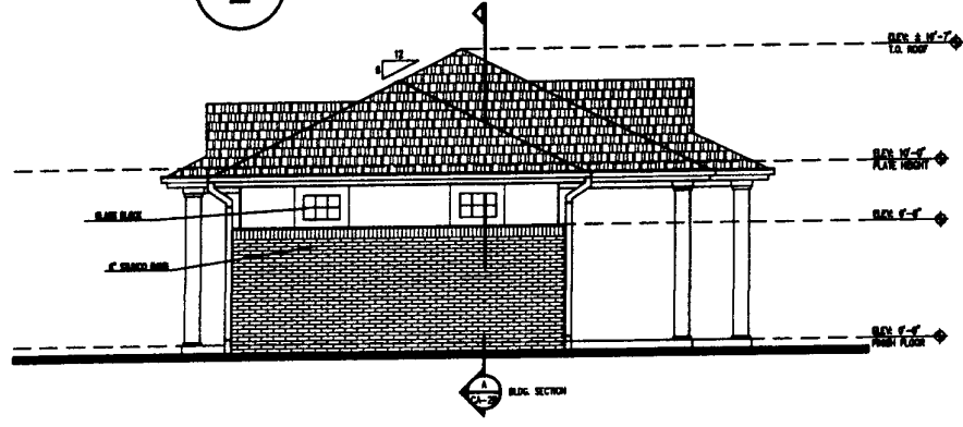
3/32" = 1'-0" 1 EAST AND WEST ELEVATIONS
