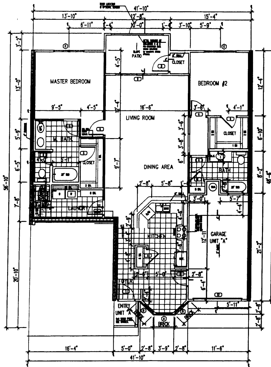
3/32" = 1'-0" 1 FIRST FLOOR PLAN UNIT A - ASHTON 2BR FLAT RIGHT UNIT 06
