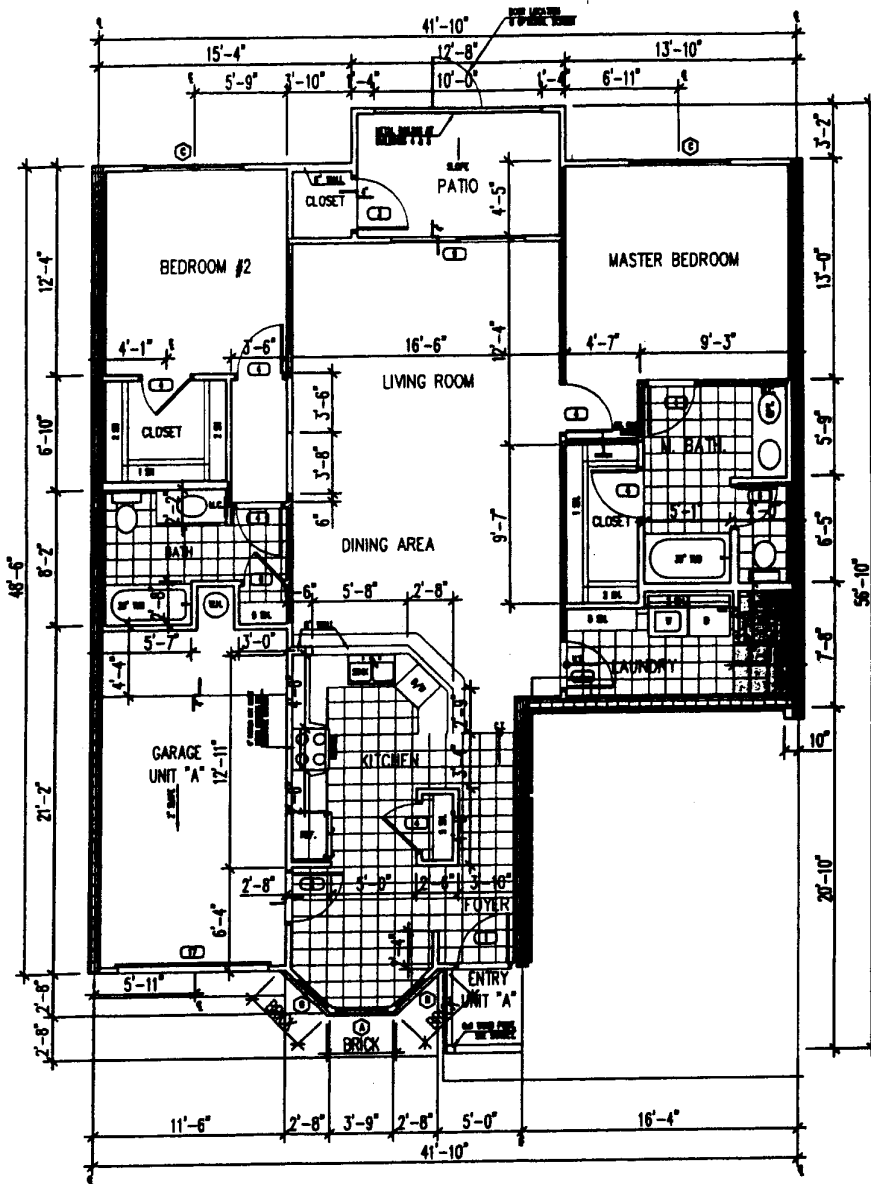
3/32"=1'-0" 1 FIRST FLOOR PLAN UNIT A - ASHTON 2BR FLAT LEFT UNIT 03
